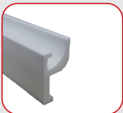
Stuckleiste 0107 BxHxL: 115x66,5x2000mm
