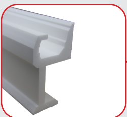
Stuckleiste 0104 BxHxL: 186x100x2000mm
